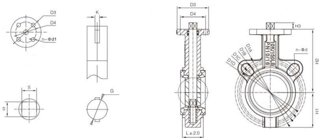
PN10&PN16&150LB&10K
